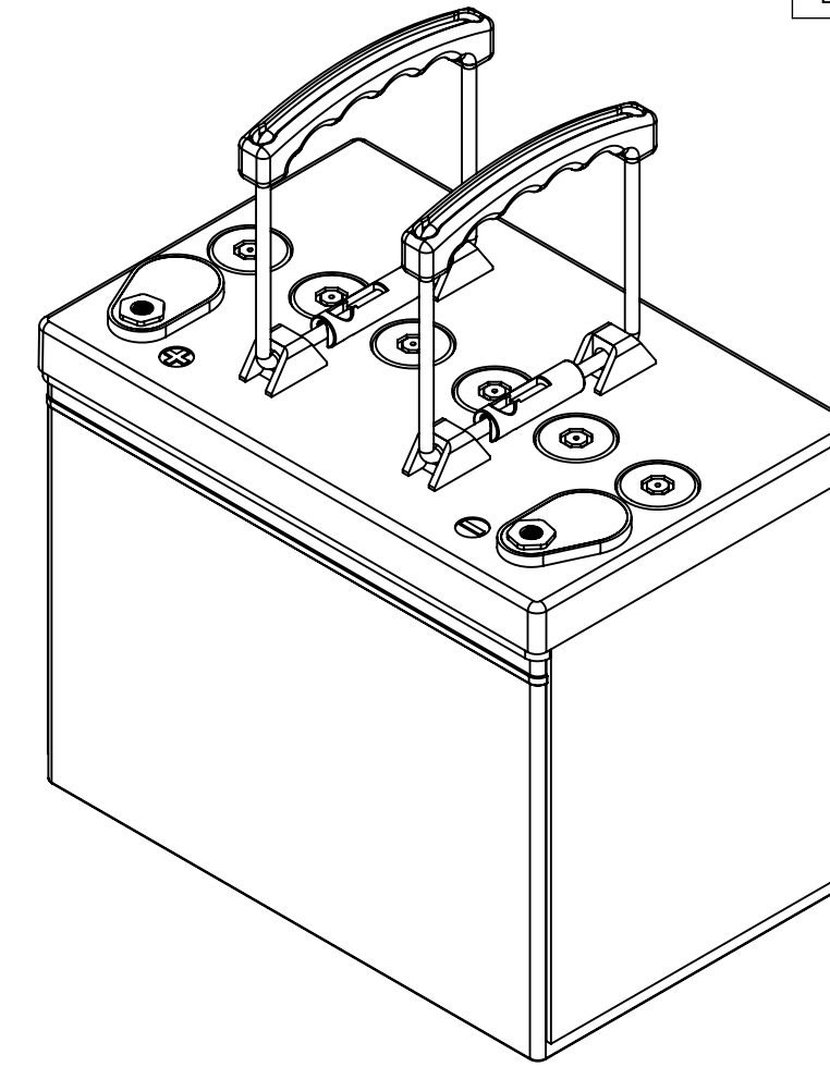
ISOMETRIC VIEW
