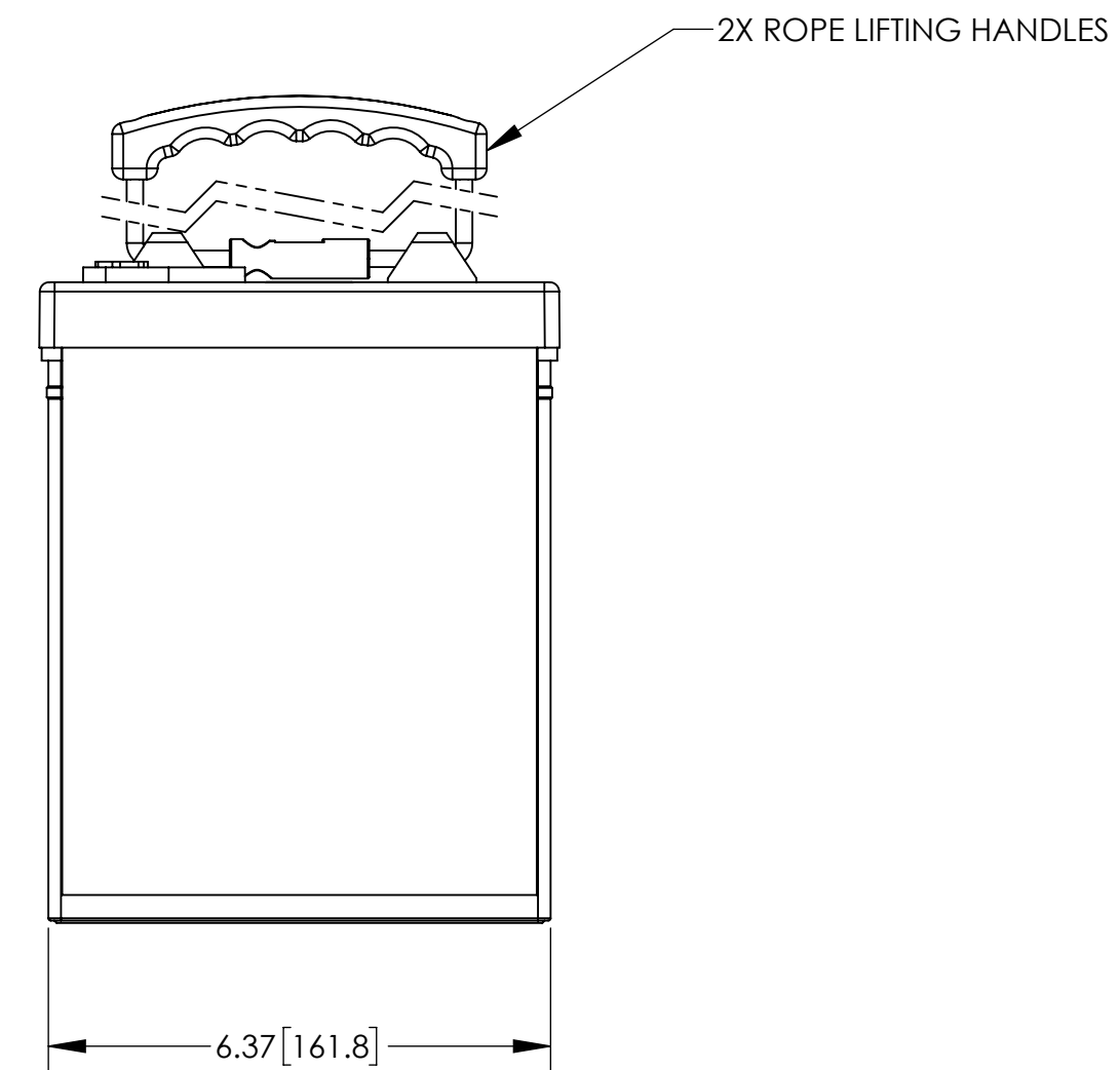
ENVELOPE DRAWING
